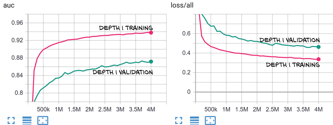
Figure 14.10 AUC (left) and loss (right) for the fine-tuning of the last linear layer
