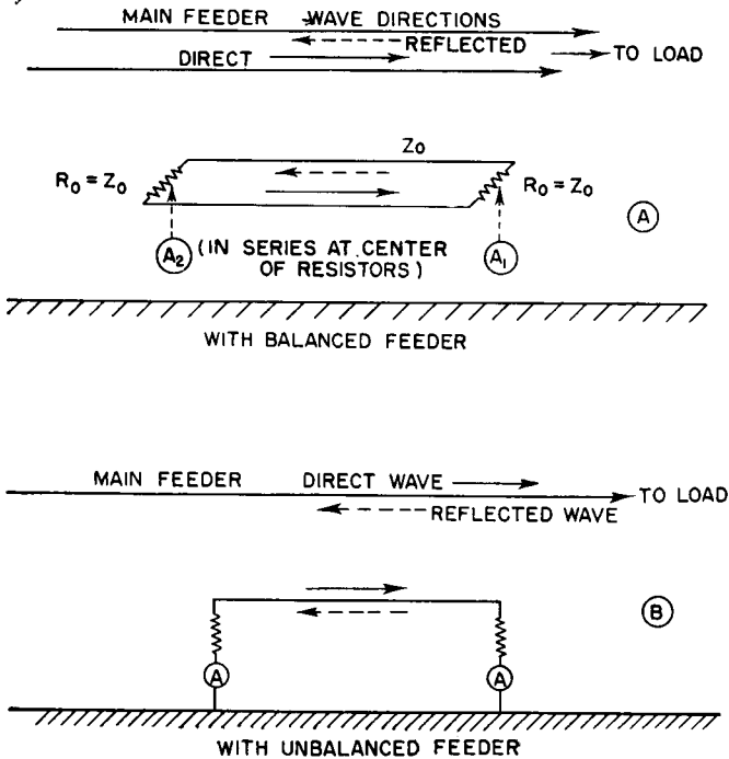
Fig. 4.62. Standing-wave indicators.
