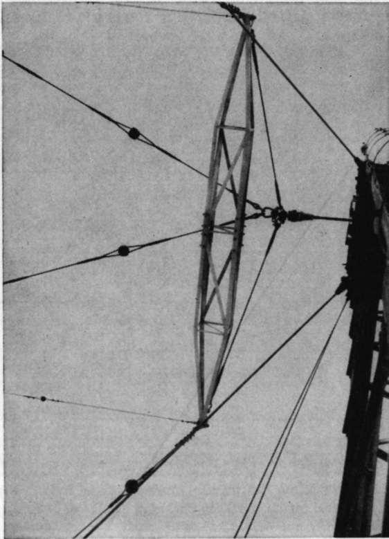
FIG. 3.102. Detail of the top of one tower supporting a high-gain dipole array, showing the cable yoke and the spreader for radiator- and reflector-curtain spacing in the main catenary. The spreader is used to space the side catenary for supporting the ends of the dipoles for the 25-meter array. (Photograph courtesy of Canadian Broadcasting Corporation.)
